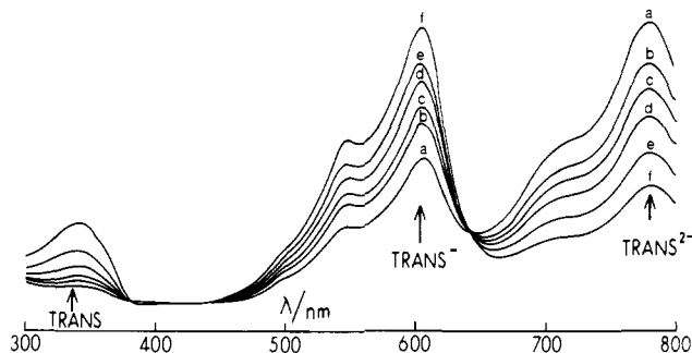
Figure 7. Typical spectra of THF solution of C + B^-, Na^+ .
